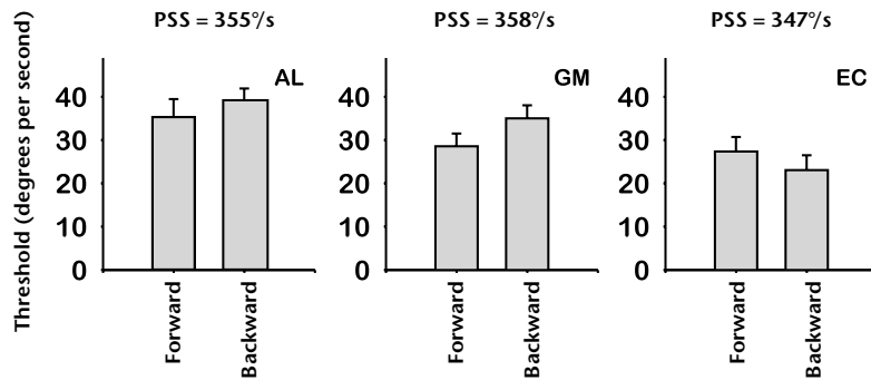
Fig. 3. Direction discrimination experiment. Thresholds for perceiving motion either in the direction of the saccade (forward) or in the opposite direction (backward). Forward and backward thresholds respectively correspond to grating speeds larger and smaller than the average saccadic peak velocity.
