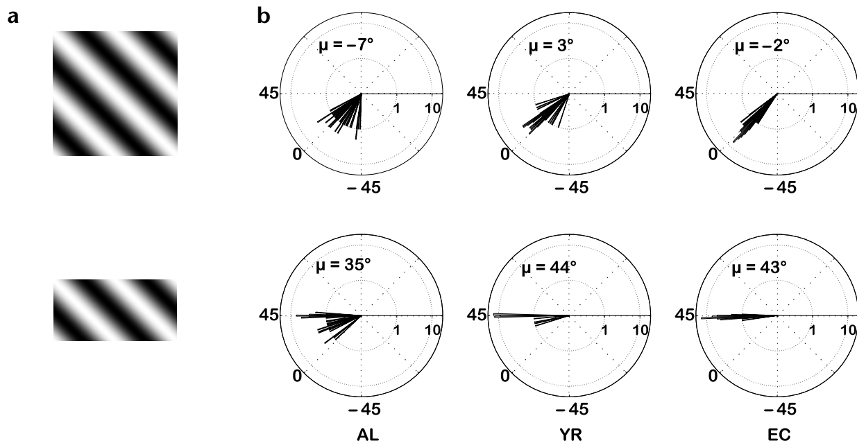
Fig. 5. Perceived direction of two-dimensional motion. (a) Stimuli were oblique ( 45^\circ ) moving gratings (contrast 30%; temporal frequency as before) presented within square ( 20^\circ \times 20^\circ ) or rectangular ( 20^\circ \times 10^\circ ) apertures. As before, observers made horizontal saccades of optimal amplitude and then rotated an arrow in the middle of the screen to indicate the direction of perceived intrasaccadic motion. (b) Distributions of perceived directions in polar coordinates. The origin ( 0^\circ ) of the angular axis represents the motion component perpendicular to the bars of the grating. The radial axis plots, in log coordinates, the number of observations collected for each direction. Mean direction is given by \mu . With a square aperture, perceived directions cluster around the perpendicular component. With a rectangular aperture, perceived directions are parallel to the long axis (barber-pole illusion).
