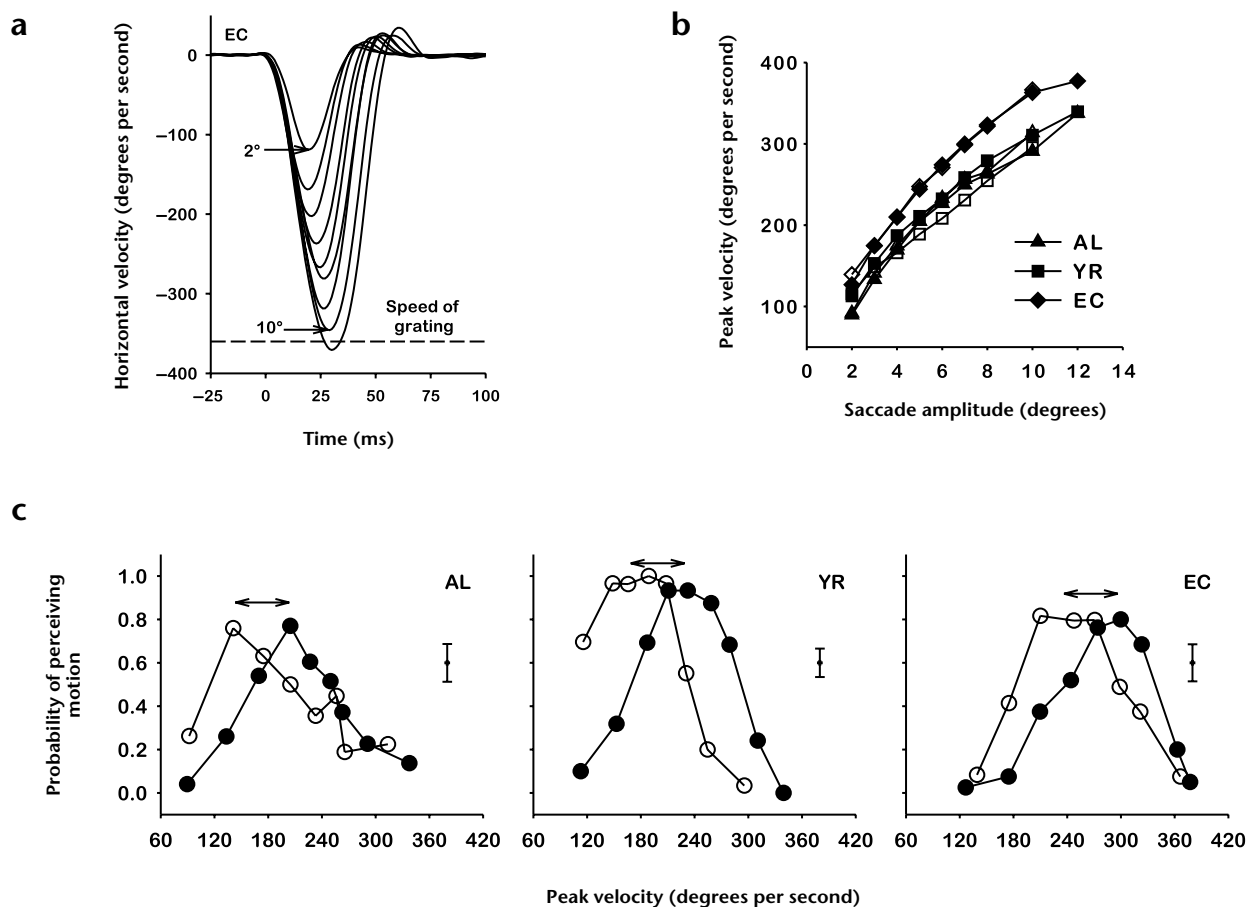
Fig. 1. Motion perception during a saccade in the same direction as a high-speed vertical grating (10% contrast). (a) Eye speed during leftward saccades (observer EC) as a function of time and saccade amplitude. Dashed line shows constant speed of a leftward-moving grating. For each saccade amplitude (two indicated by arrows), the mean velocity profile was obtained from aligning onsets of individual saccades and averaging their velocity profiles. (b) Dependence of peak velocity on saccade amplitude. For each combination of saccade amplitude and grating speed (solid symbols, 360° per s; open symbols, 300° per s), we measured the mean saccadic peak velocity by averaging individual peak velocities. (c) Probability of perceiving motion as a function of saccadic peak velocity for three observers. Gratings moving at either 360° per s (filled symbols) or 300° per s (open symbols) were presented in successive blocks. Error bars to right show average s.e. For all observers, the two inverted U-shaped curves were laterally shifted by 60° per s (horizontal arrows).
