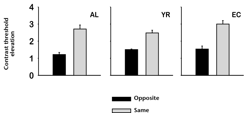
Fig. 4. Direction-selective adaptation. Observers made horizontal saccades and detected whether a horizontally moving test grating was located in the top or bottom half of the screen (spatial 2AFC). Contrast sensitivity was measured with or without adaptation to a moving grating. The data clearly show direction-selective adaptation: contrast-threshold elevation (relative to the unadapted condition) was larger when the adapting grating was in the same rather than in the opposite direction.
